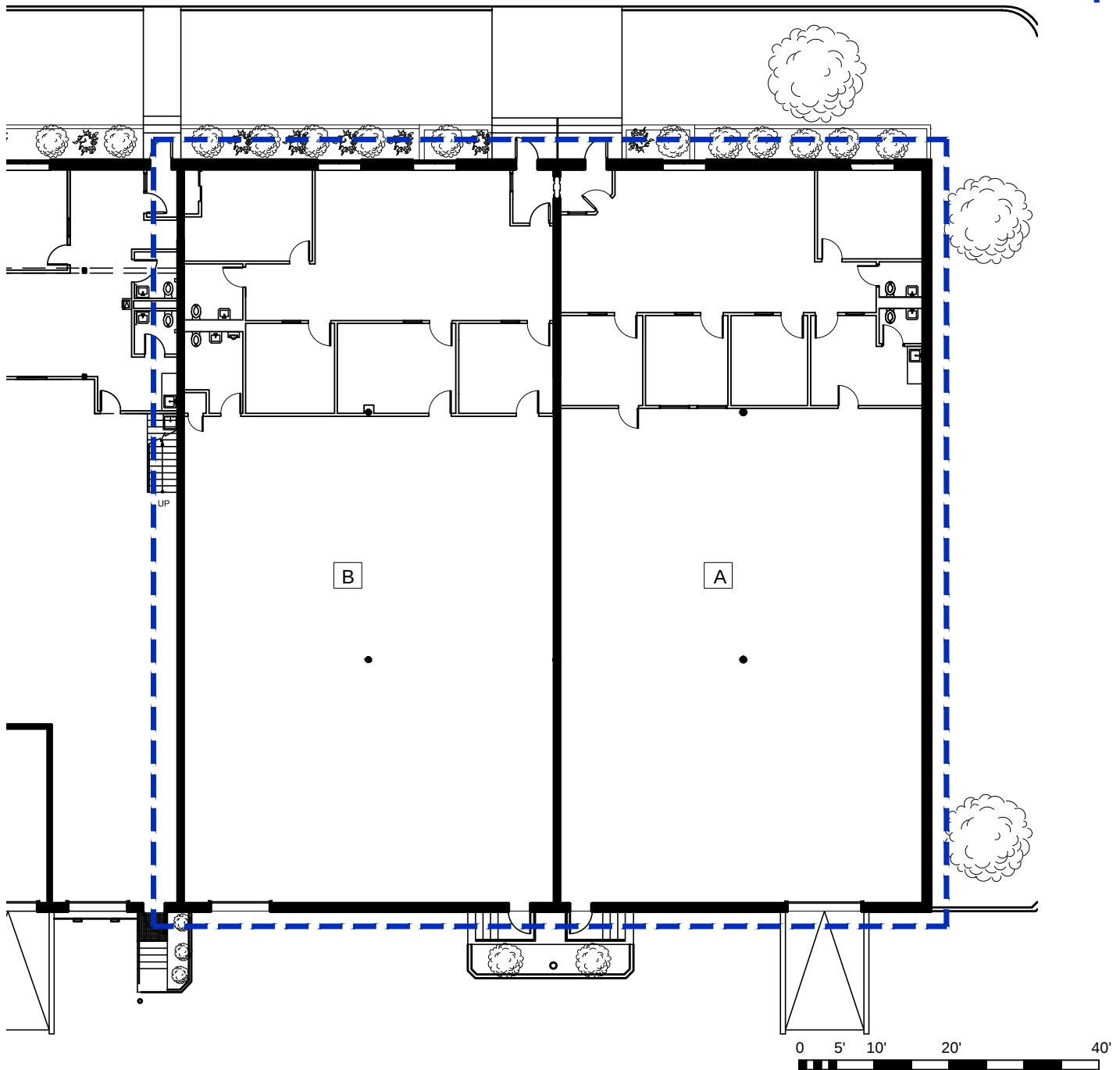
GENERIC LEASE PLAN
